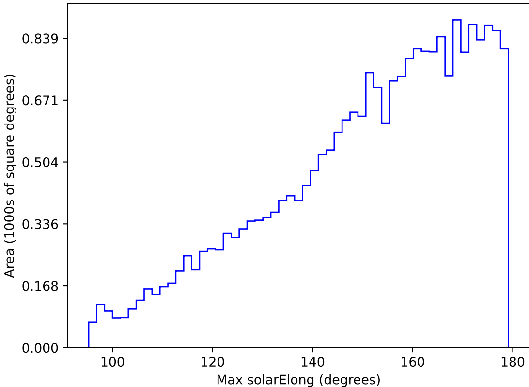
baseline_v2.0_10yrs All sky u band: Max solarElong
