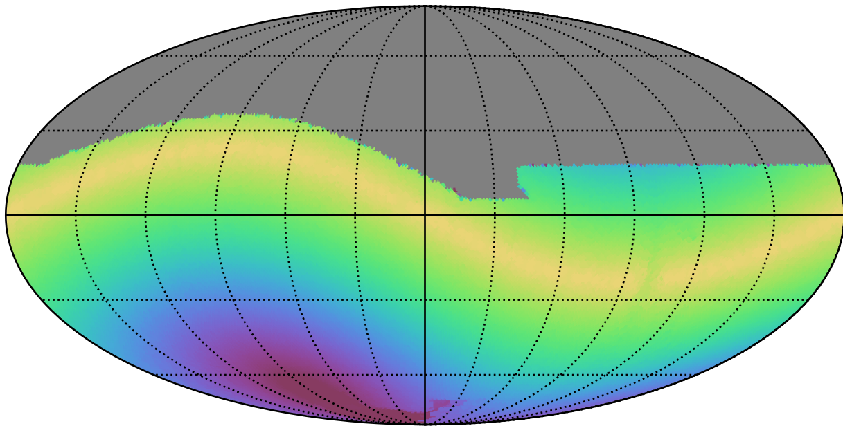
baseline_v2.0_10yrs All sky r band: Max solarElong
