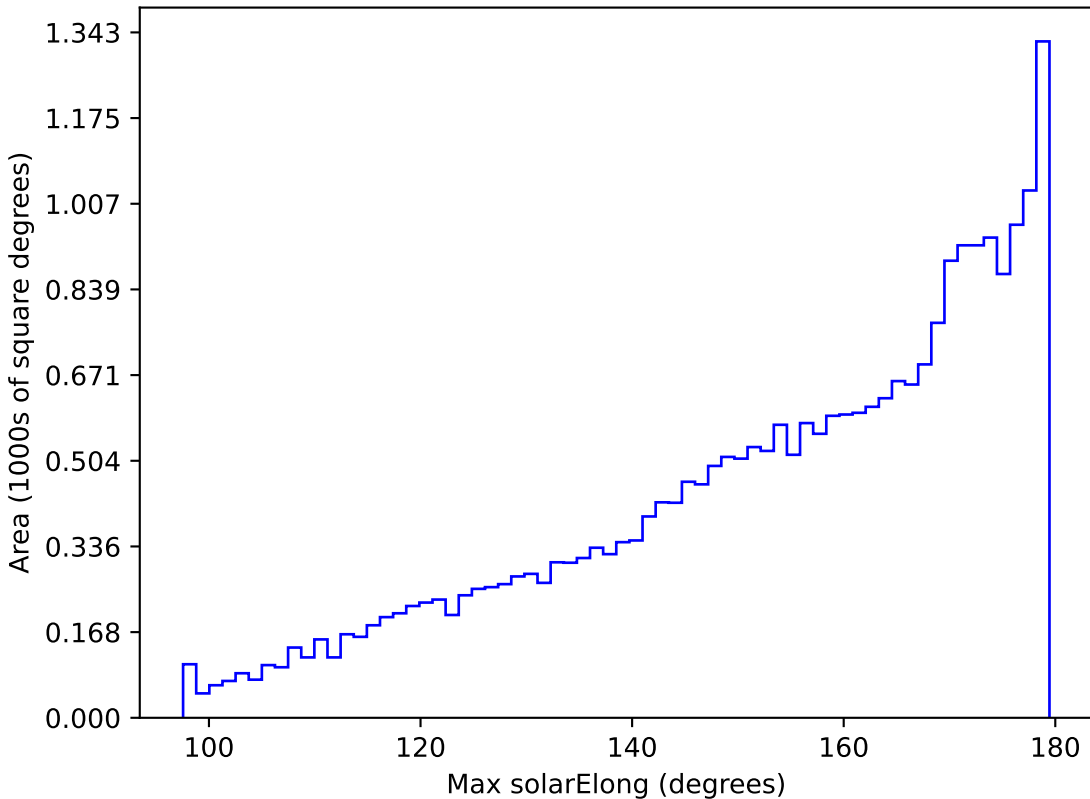
baseline_v2.0_10yrs All sky r band: Max solarElong
