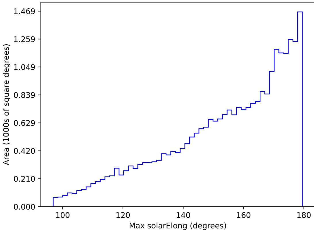
baseline_v2.0_10yrs All sky i band: Max solarElong
