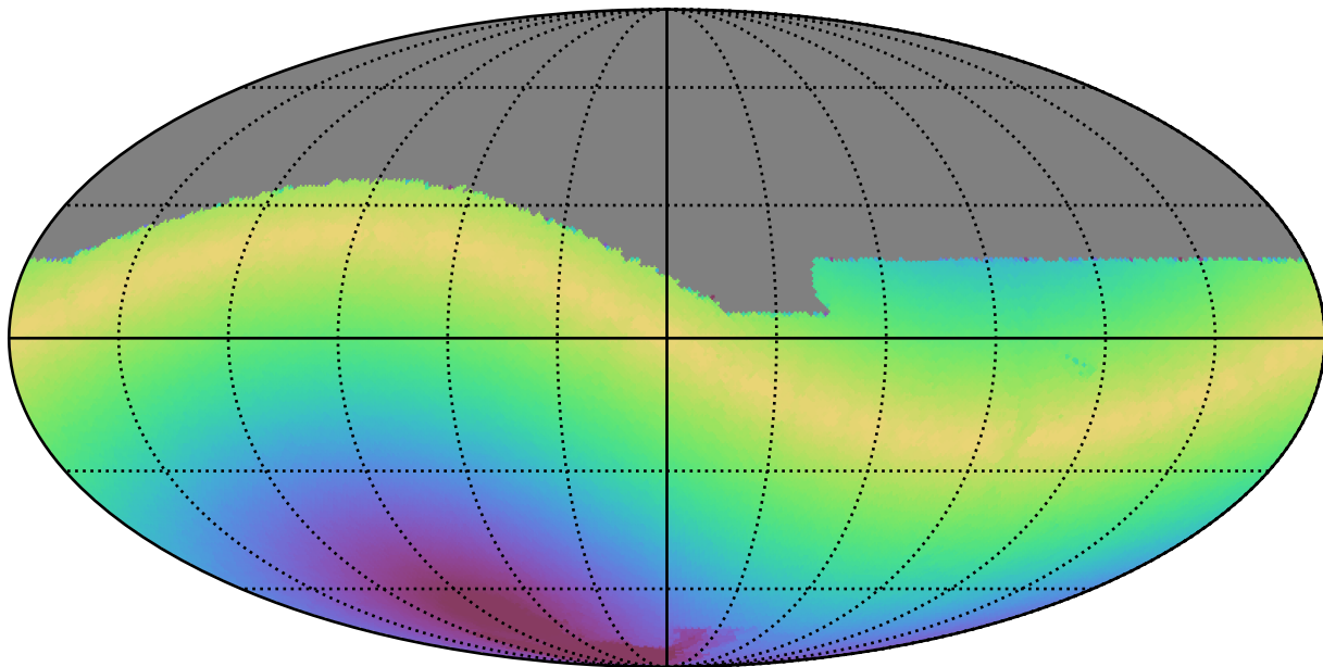
baseline_v2.0_10yrs All sky g band: Max solarElong
