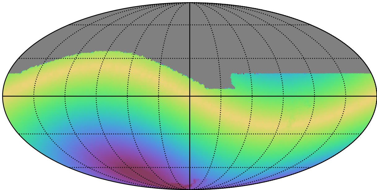
baseline_v2.0_10yrs All sky all bands: Max solarElong
