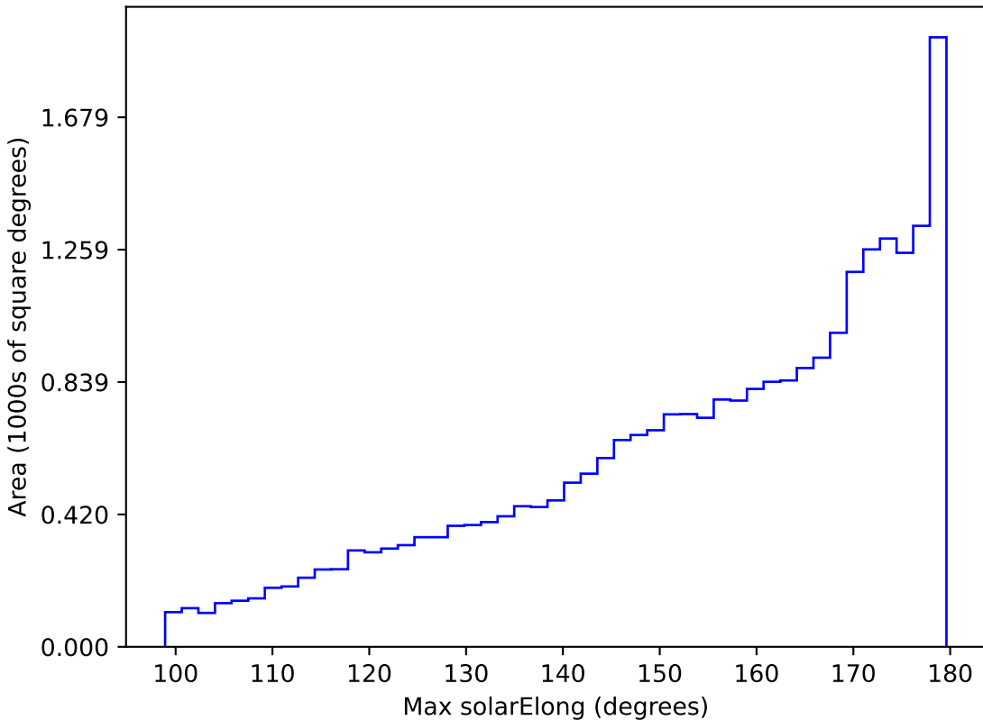
baseline_v2.0_10yrs All sky all bands: Max solarElong
