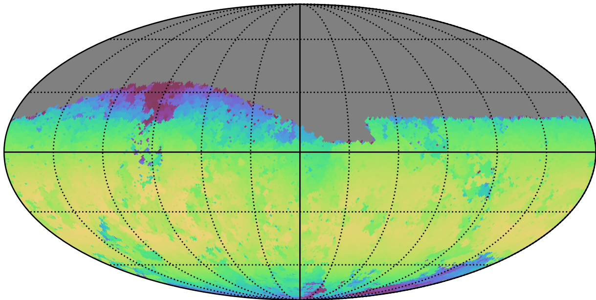
baseline_v2.0_10yrs Yr 1 z band: Max skyBrightness
