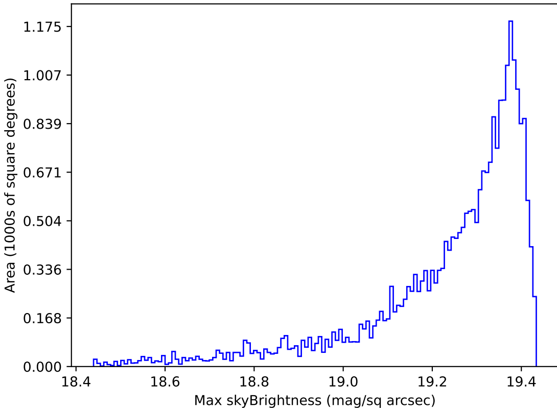
baseline_v2.0_10yrs Yr 1 z band: Max skyBrightness
