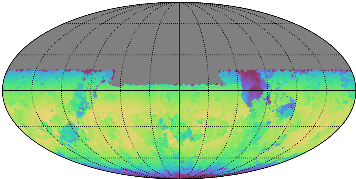
baseline_v2.0_10yrs Yr 1 y band: Max skyBrightness
