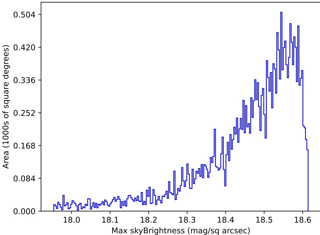
baseline_v2.0_10yrs Yr 1 y band: Max skyBrightness
