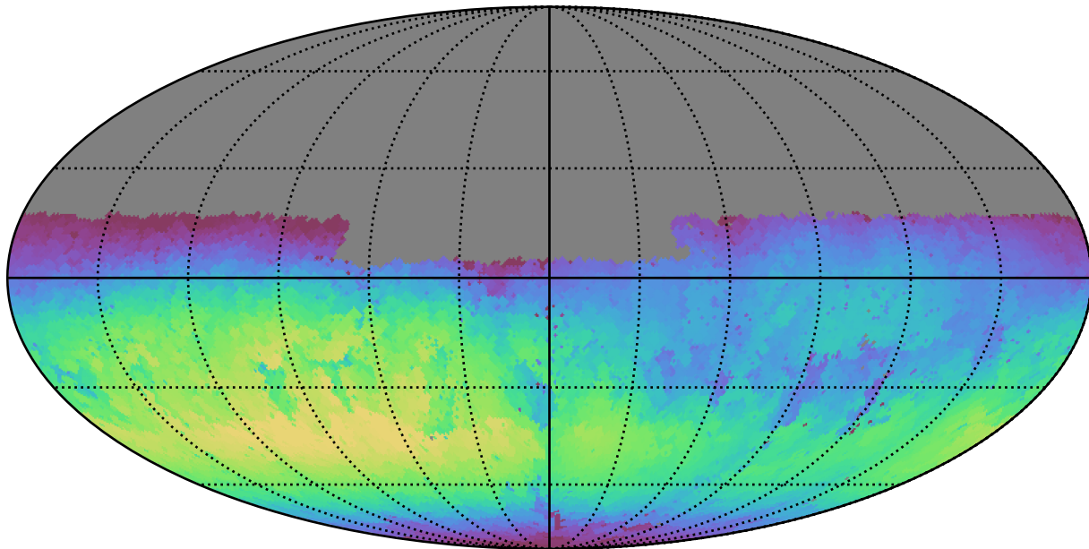
baseline_v2.0_10yrs Yr 1 u band: Max skyBrightness
