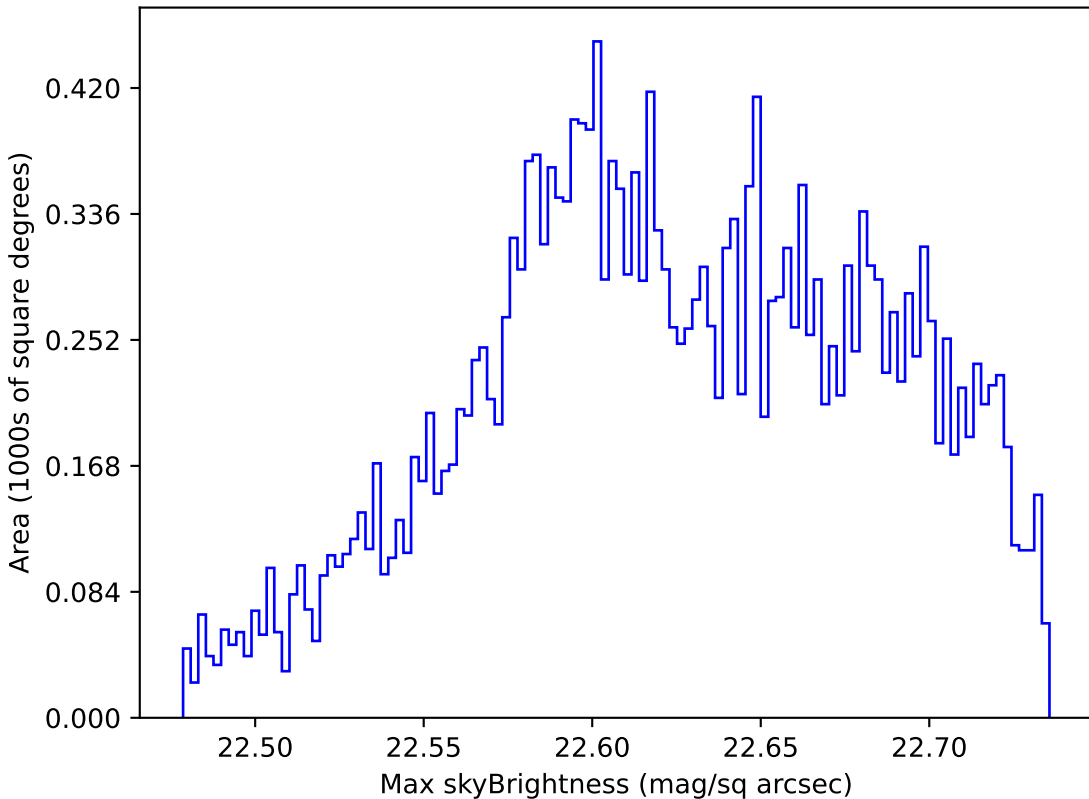
baseline_v2.0_10yrs Yr 1 u band: Max skyBrightness
