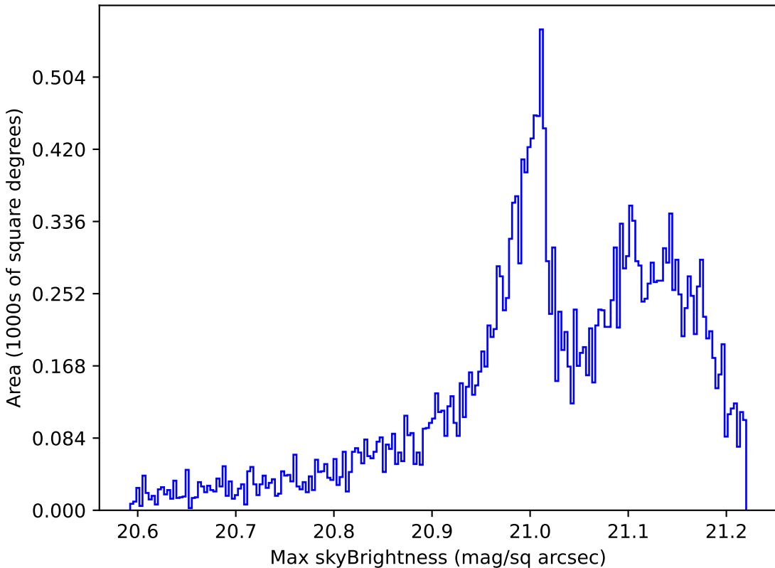
baseline_v2.0_10yrs Yr 1 r band: Max skyBrightness
