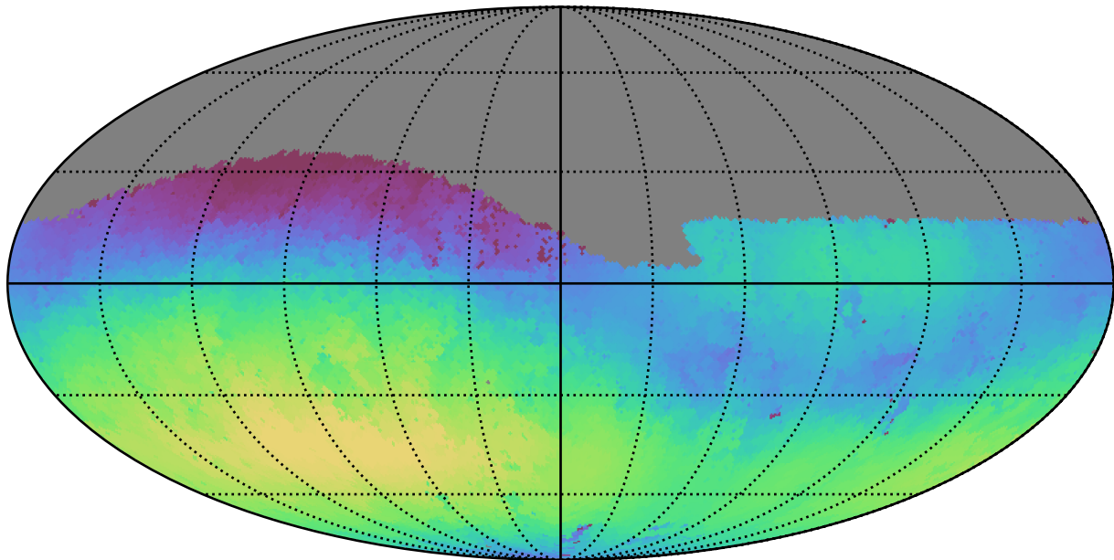
baseline_v2.0_10yrs Yr 1 g band: Max skyBrightness
