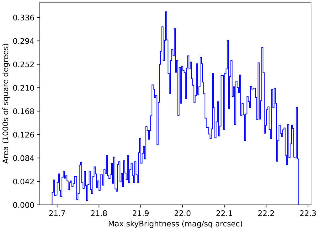
baseline_v2.0_10yrs Yr 1 g band: Max skyBrightness
