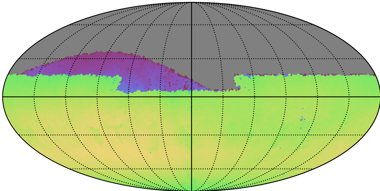
baseline_v2.0_10yrs Yr 1 all bands: Max skyBrightness
