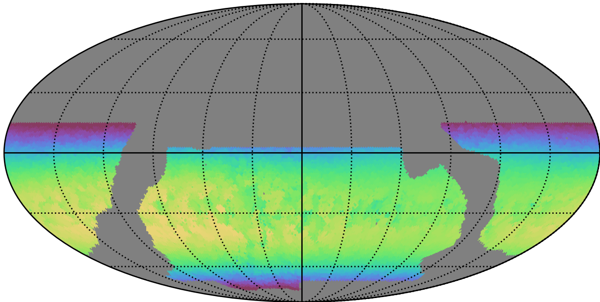
baseline_v2.0_10yrs WFD z band: Max skyBrightness
