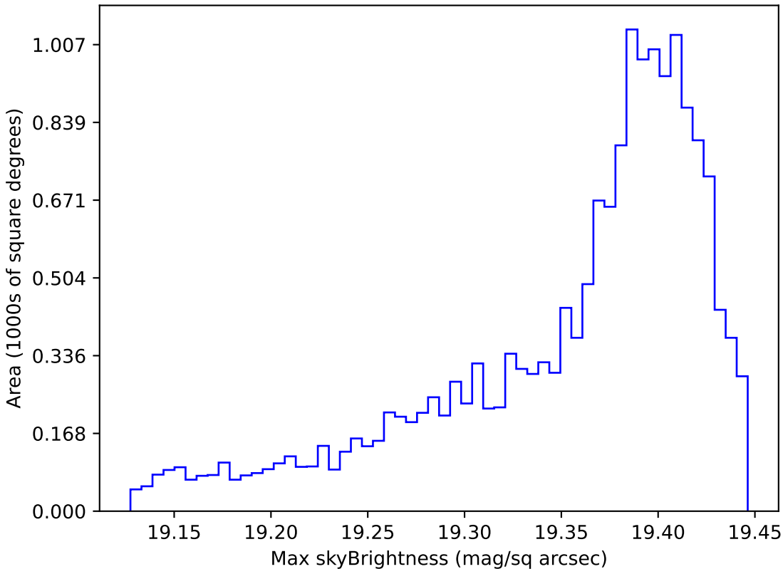
baseline_v2.0_10yrs WFD z band: Max skyBrightness
