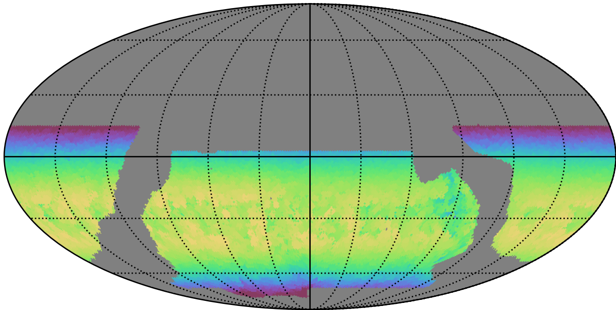
baseline_v2.0_10yrs WFD y band: Max skyBrightness
