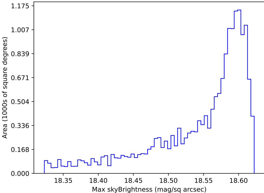
baseline_v2.0_10yrs WFD y band: Max skyBrightness
