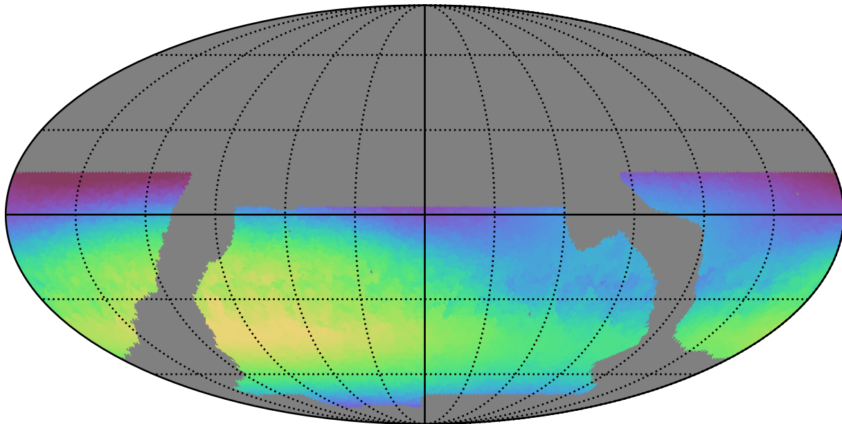
baseline_v2.0_10yrs WFD u band: Max skyBrightness
