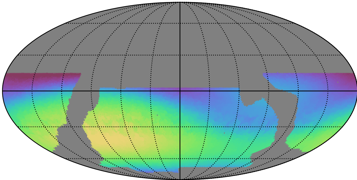
baseline_v2.0_10yrs WFD r band: Max skyBrightness
