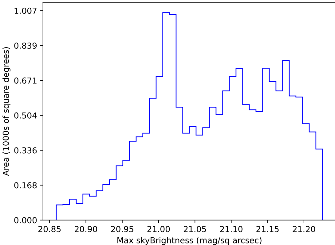
baseline_v2.0_10yrs WFD r band: Max skyBrightness
