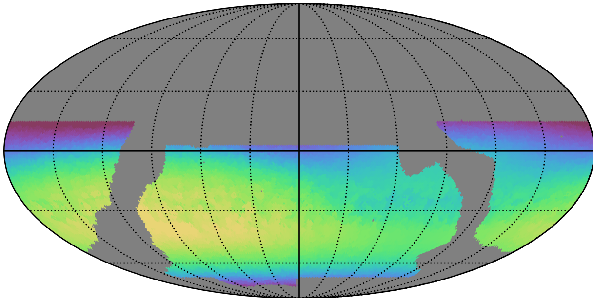
baseline_v2.0_10yrs WFD i band: Max skyBrightness
