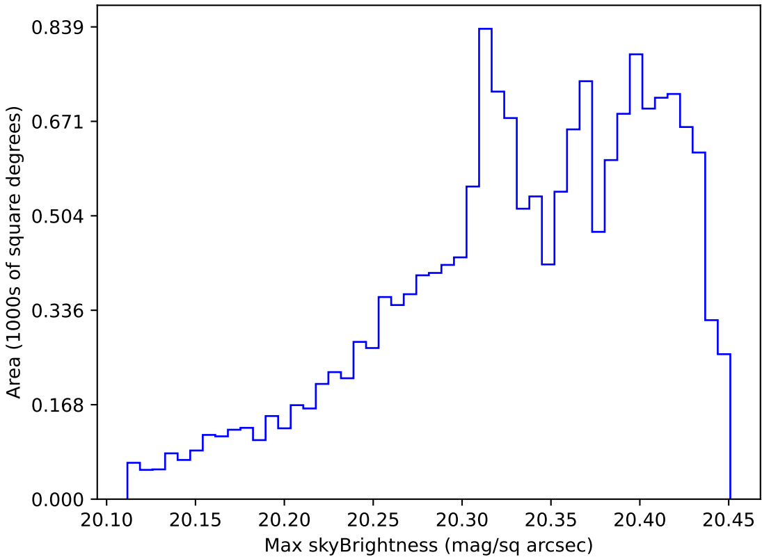
baseline_v2.0_10yrs WFD i band: Max skyBrightness
