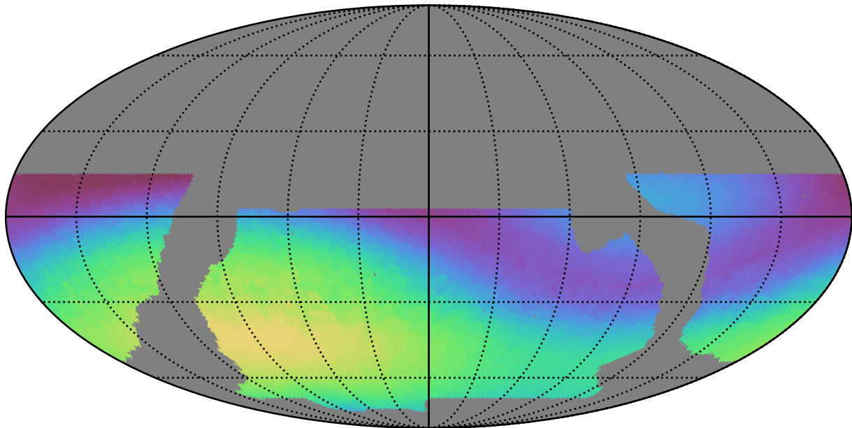
baseline_v2.0_10yrs WFD g band: Max skyBrightness
