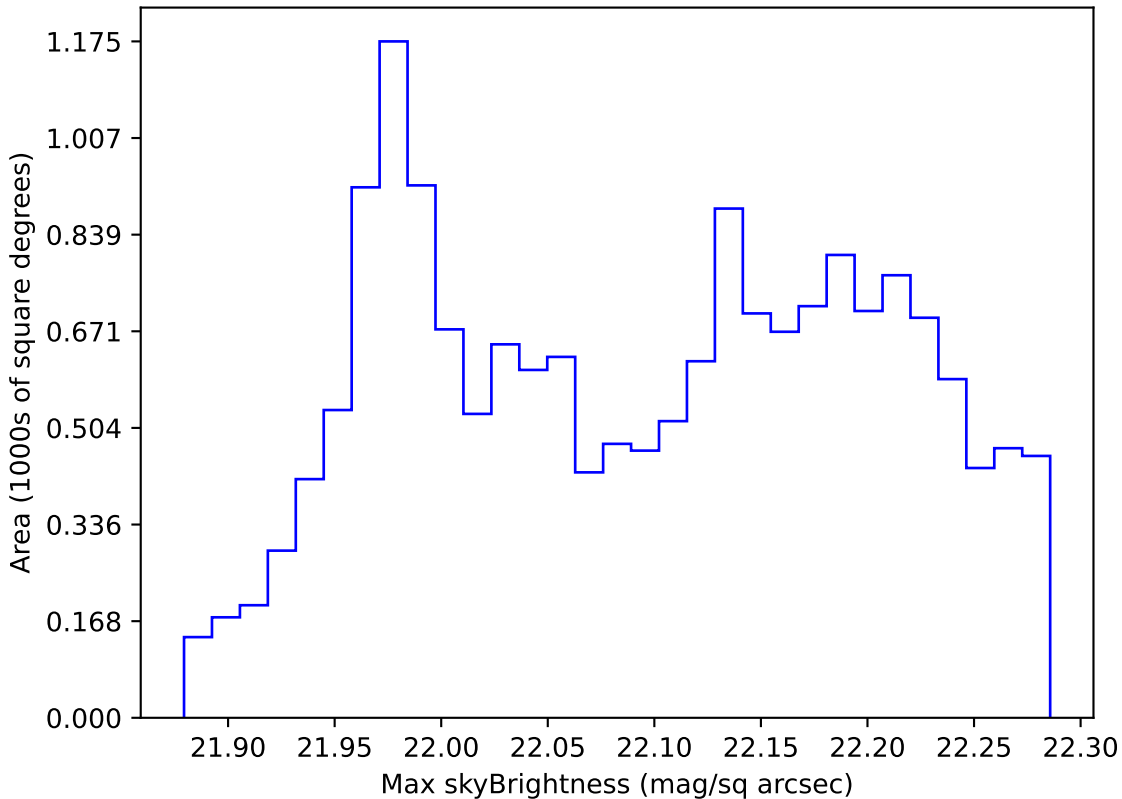
baseline_v2.0_10yrs WFD g band: Max skyBrightness
