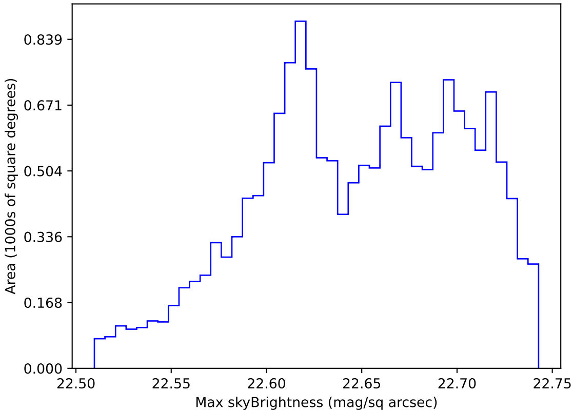
baseline_v2.0_10yrs WFD all bands: Max skyBrightness
