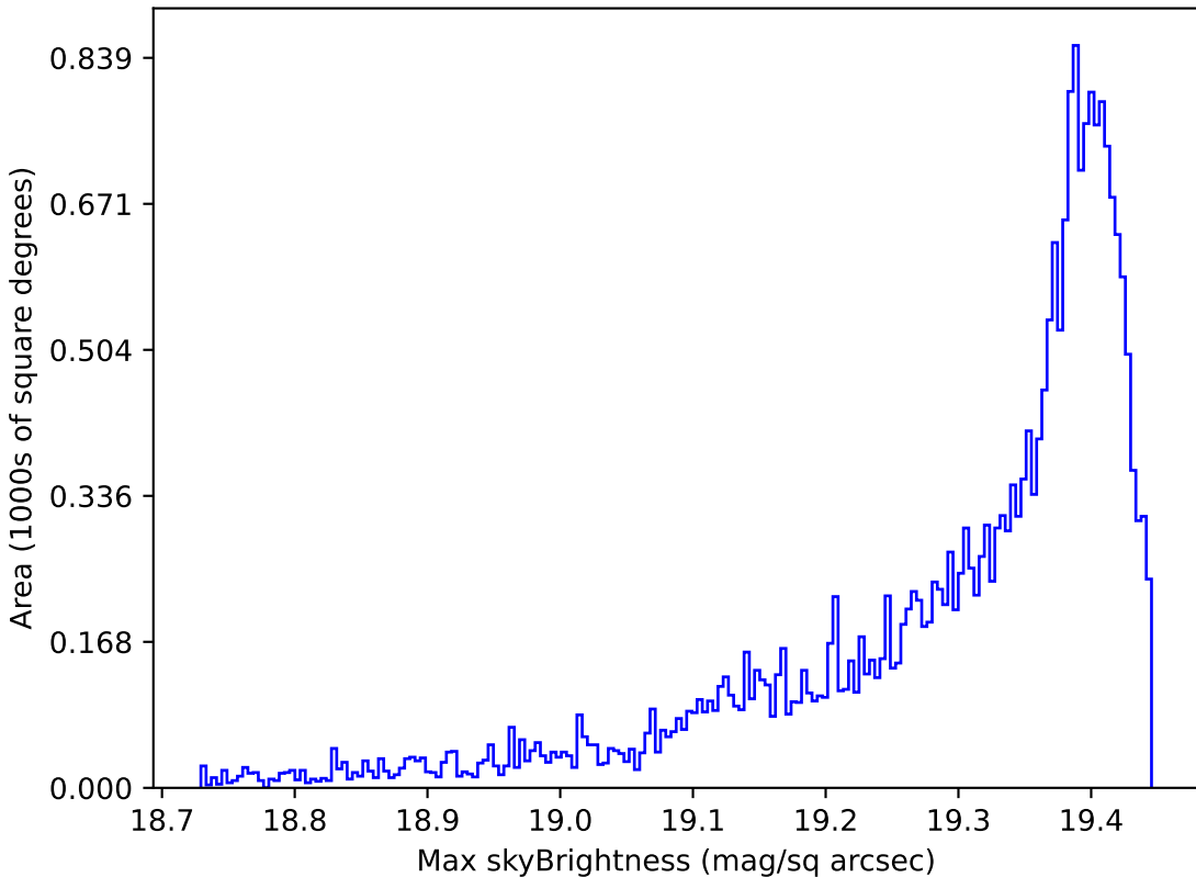
baseline_v2.0_10yrs All sky z band: Max skyBrightness
