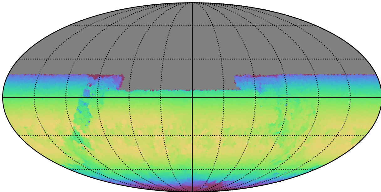
baseline_v2.0_10yrs All sky y band: Max skyBrightness
