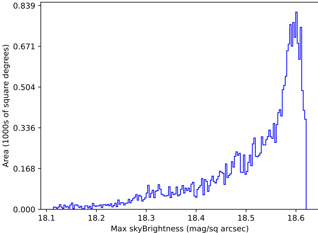
baseline_v2.0_10yrs All sky y band: Max skyBrightness
