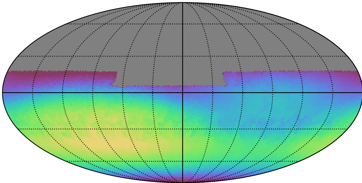
baseline_v2.0_10yrs All sky u band: Max skyBrightness
