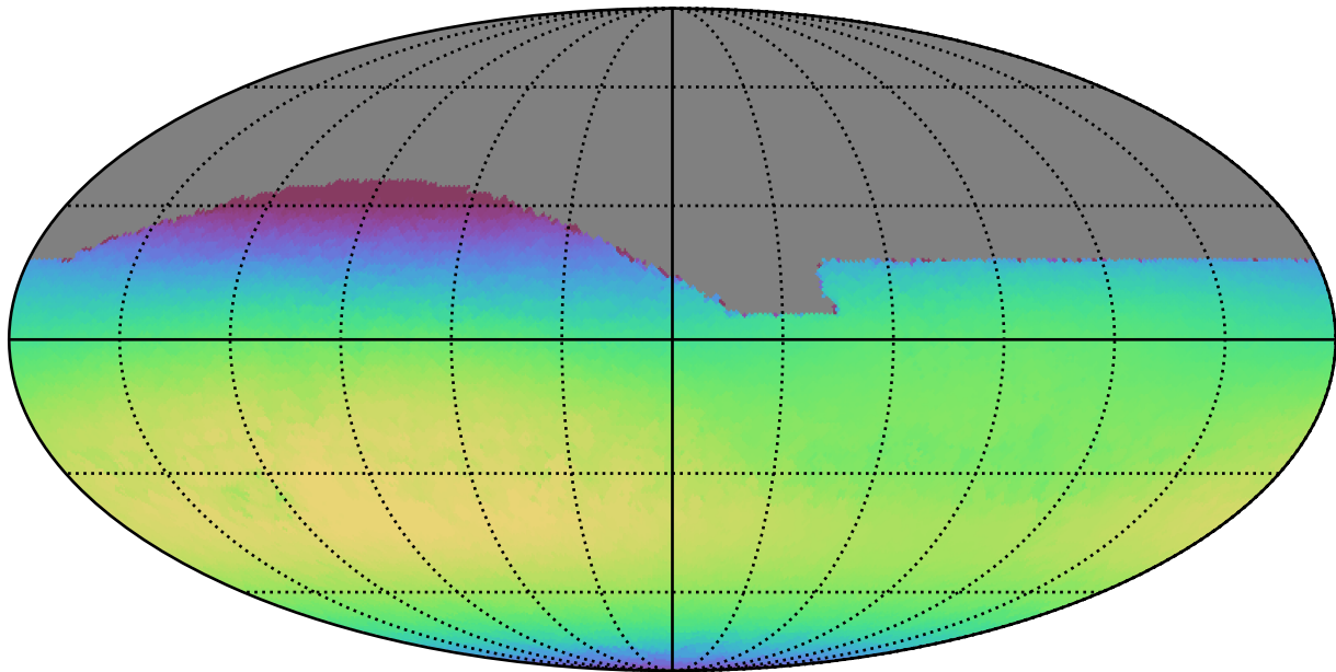
baseline_v2.0_10yrs All sky i band: Max skyBrightness
