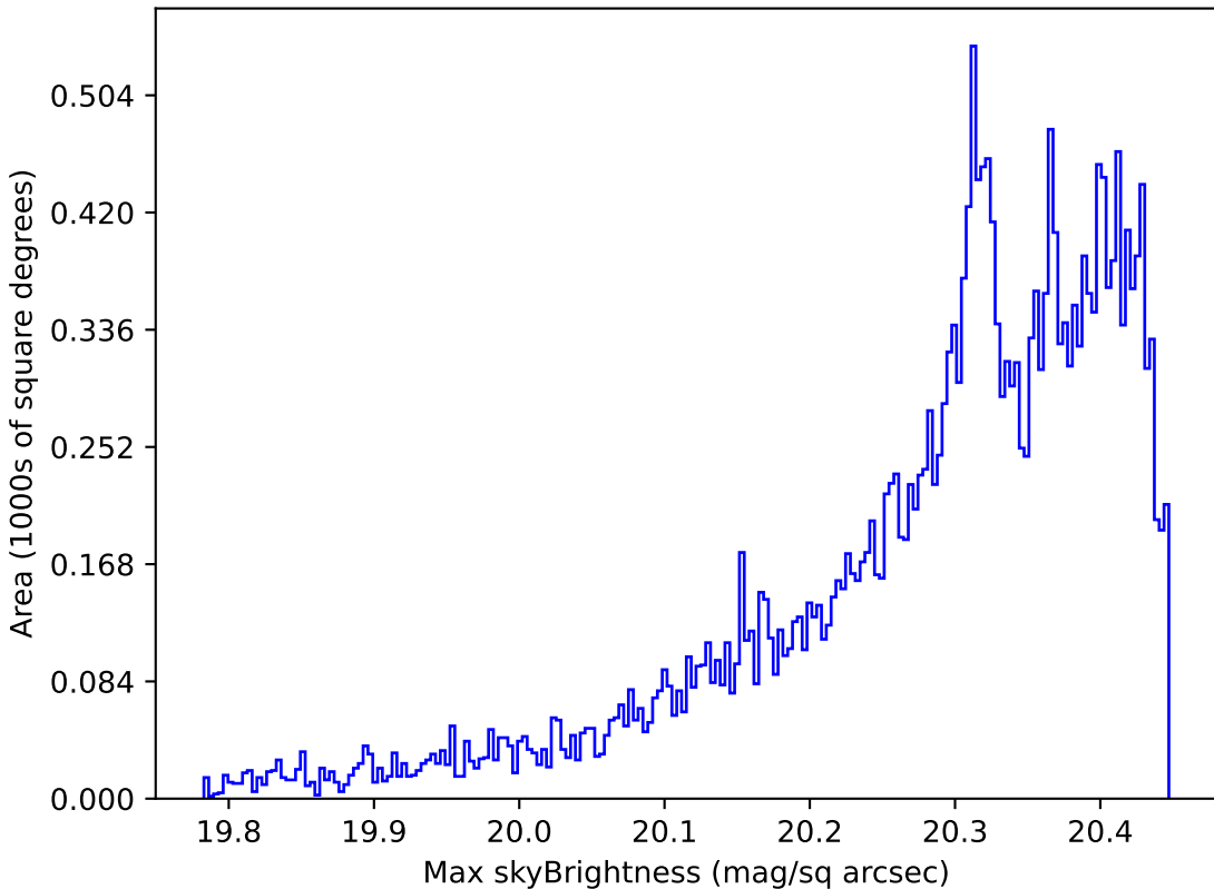
baseline_v2.0_10yrs All sky i band: Max skyBrightness
