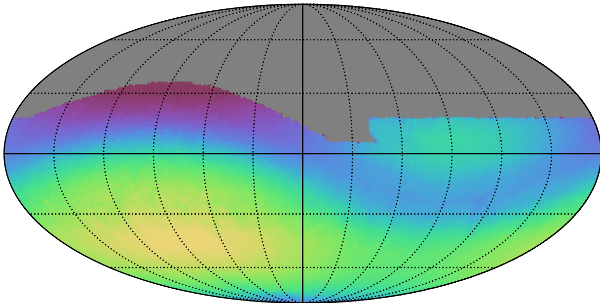
baseline_v2.0_10yrs All sky g band: Max skyBrightness
