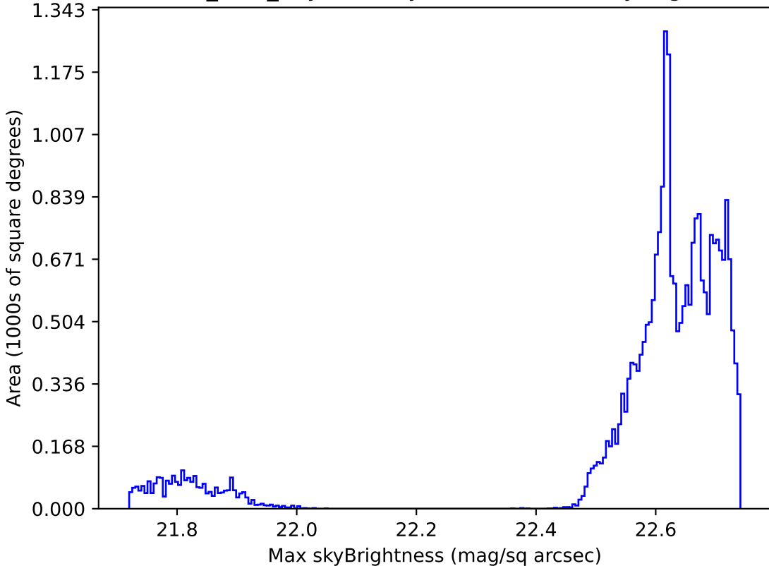
baseline_v2.0_10yrs All sky all bands: Max skyBrightness
