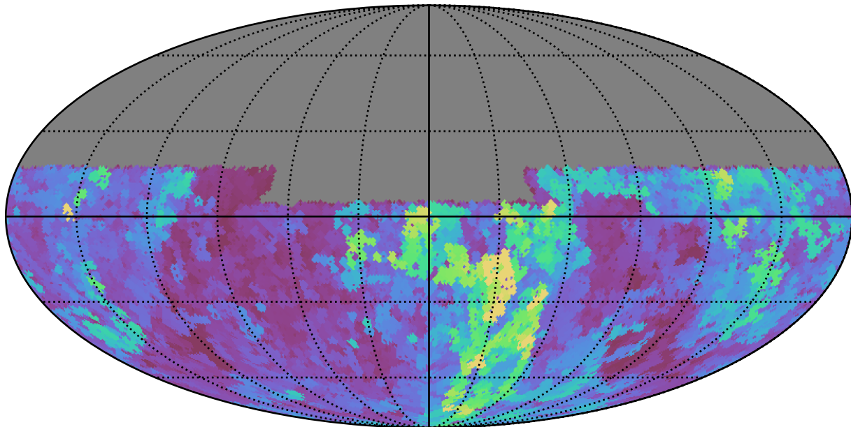
baseline_v2.0_10yrs Yr 1 y band: Max seeingGeom
