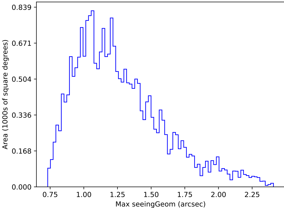
baseline_v2.0_10yrs Yr 1 y band: Max seeingGeom
