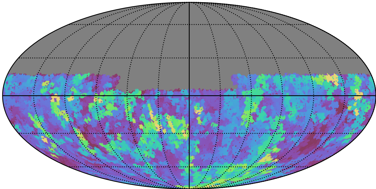
baseline_v2.0_10yrs Yr 1 u band: Max seeingGeom
