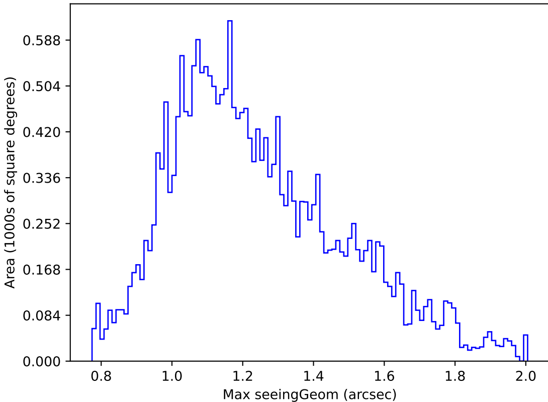
baseline_v2.0_10yrs Yr 1 u band: Max seeingGeom
