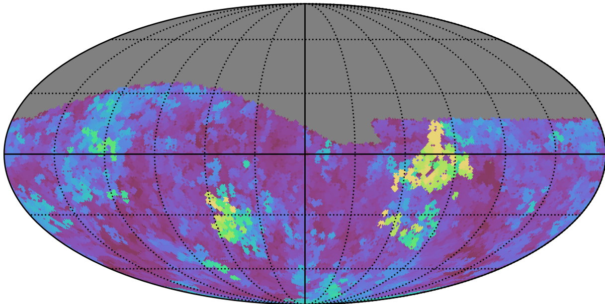
baseline_v2.0_10yrs Yr 1 r band: Max seeingGeom
