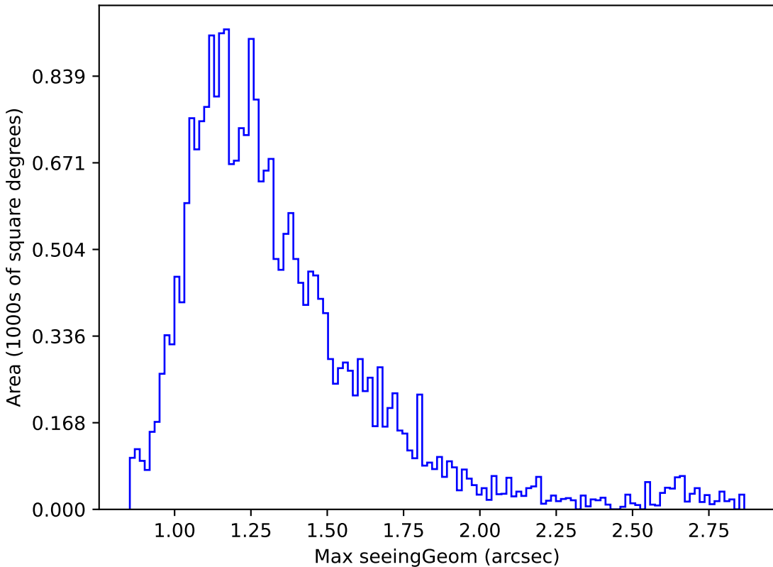
baseline_v2.0_10yrs Yr 1 r band: Max seeingGeom
