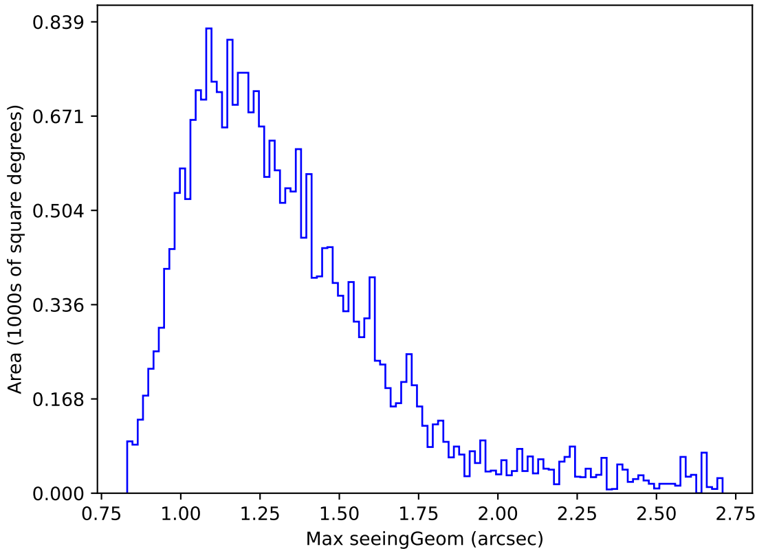
baseline_v2.0_10yrs Yr 1 i band: Max seeingGeom
