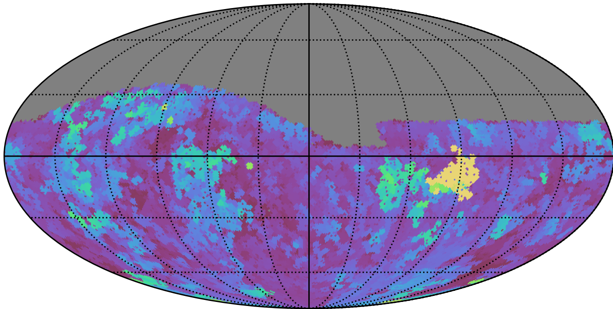
baseline_v2.0_10yrs Yr 1 g band: Max seeingGeom
