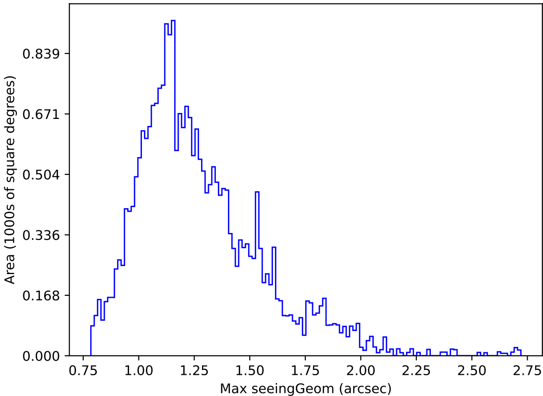
baseline_v2.0_10yrs Yr 1 g band: Max seeingGeom
