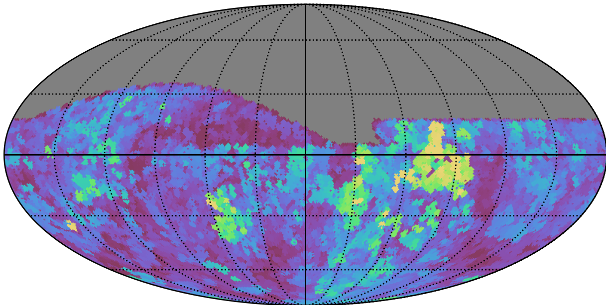
baseline_v2.0_10yrs Yr 1 all bands: Max seeingGeom
