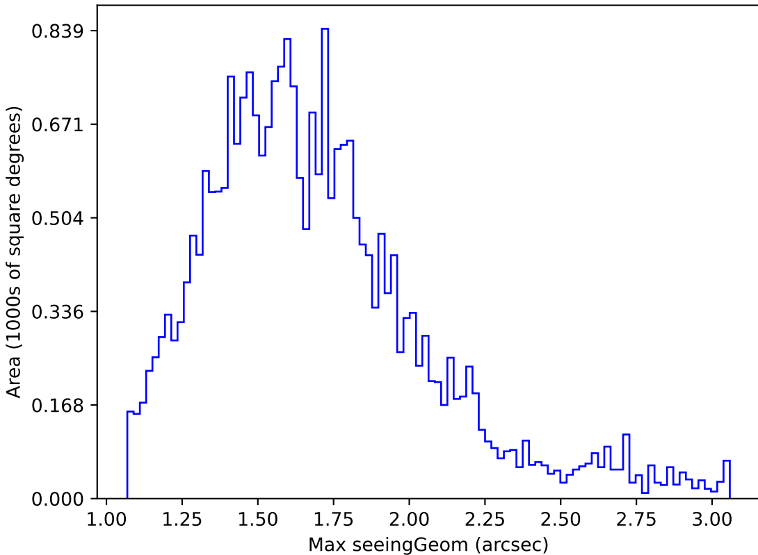
baseline_v2.0_10yrs Yr 1 all bands: Max seeingGeom
