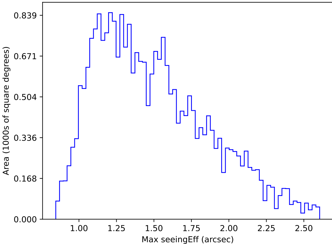
baseline_v2.0_10yrs Yr 1 z band: Max seeingEff
