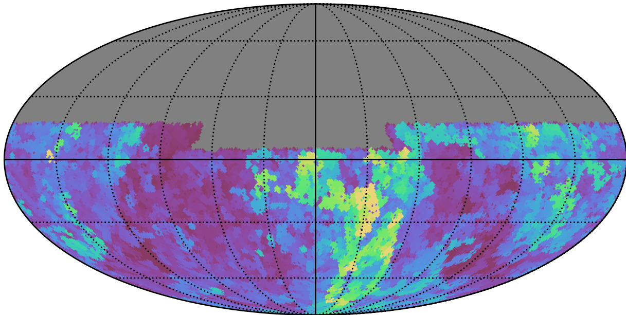
baseline_v2.0_10yrs Yr 1 y band: Max seeingEff
